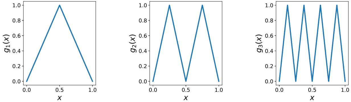
Fig. 3: Sawtooth functions
