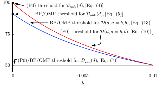
Figure 1. Deterministic sparsity thresholds guaranteeing uniqueness of (P0) and recoverability via BP and OMP for dictionaries in \mathcal{D}_{\text{gen}}(d) , \mathcal{D}_{\text{omb}}(d) , and \mathcal{D}(d, a, b) . We set d = 0.01 and consider the special case a = b . Note that for a = b , the threshold in (10) reduces to that in (11).
