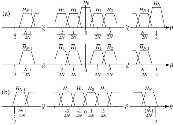
Figure 1. Transfer functions of the channel filters in (a) a WFB or, more generally, an even-stacked CMFB with 2N channels, (b) an N -channel odd-stacked CMFB.
