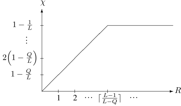
Fig. 1. The capacity pre-log of the SIMO channel (3).
